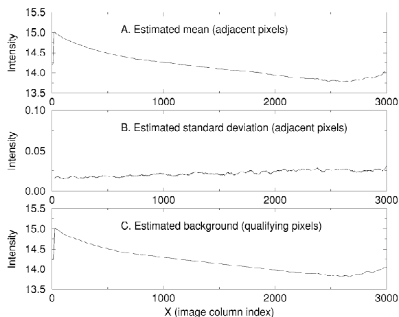
Fig. 7. Estimating the background level. (A) Initial estimate of background level (Step 2). (B) Initial estimate of background noise standard deviation (Step 2). (C) Final estimate of background level (Step 3).
